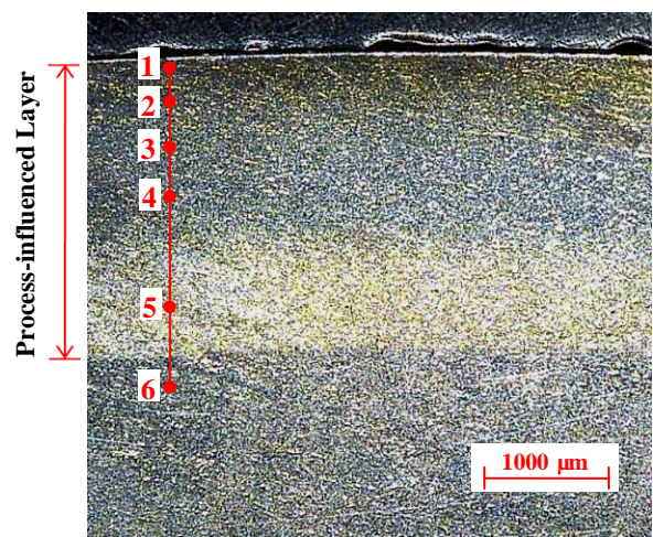
Figure 2 Microstructure after cryogenic burnishing ( \times 30 magnification)
