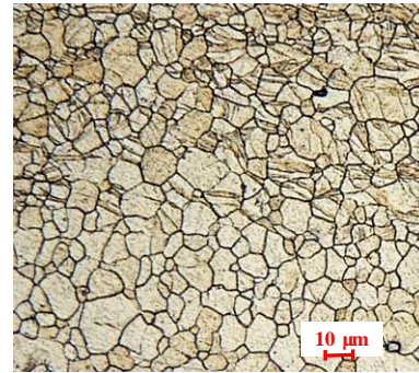
Figure 3 Interface between initial material and process-influenced layer after cryogenic burnishing ( \times 1000 magnification)
