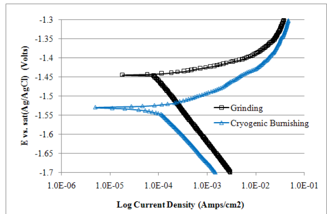
Figure 8 Polarization curves of AZ31B Mg samples after grinding and cryogenic burnishing in 5 wt.% NaCl
